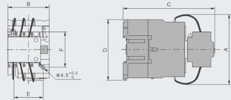
CJ19-25~43 Contactor appearance and installation dimensions
