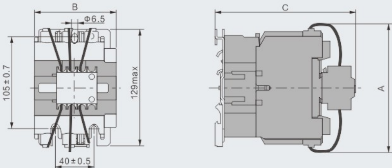
CJ19-63~95 Contactor appearance and installation dimensions
