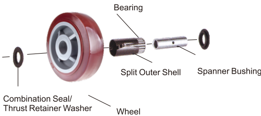
The detail sketch of wheel >
