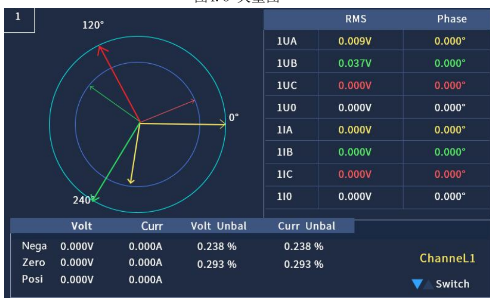
Fig. 4.8 Phasors
