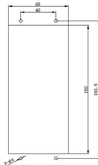
Cut-out Dimension
