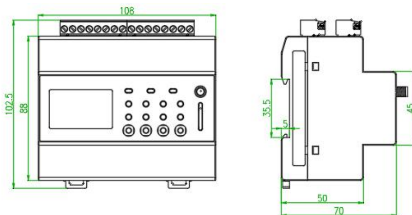
Figure 3 AMC200(L) Outline-Dimensions
