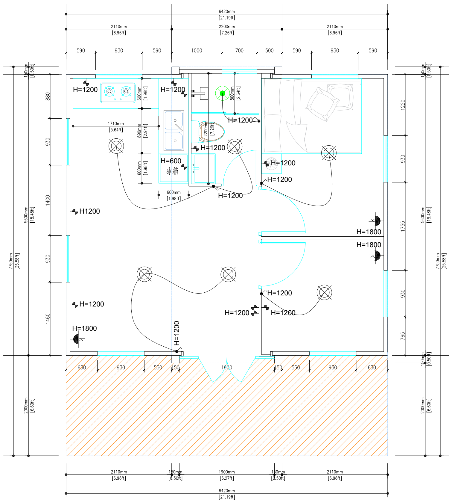
First floor
