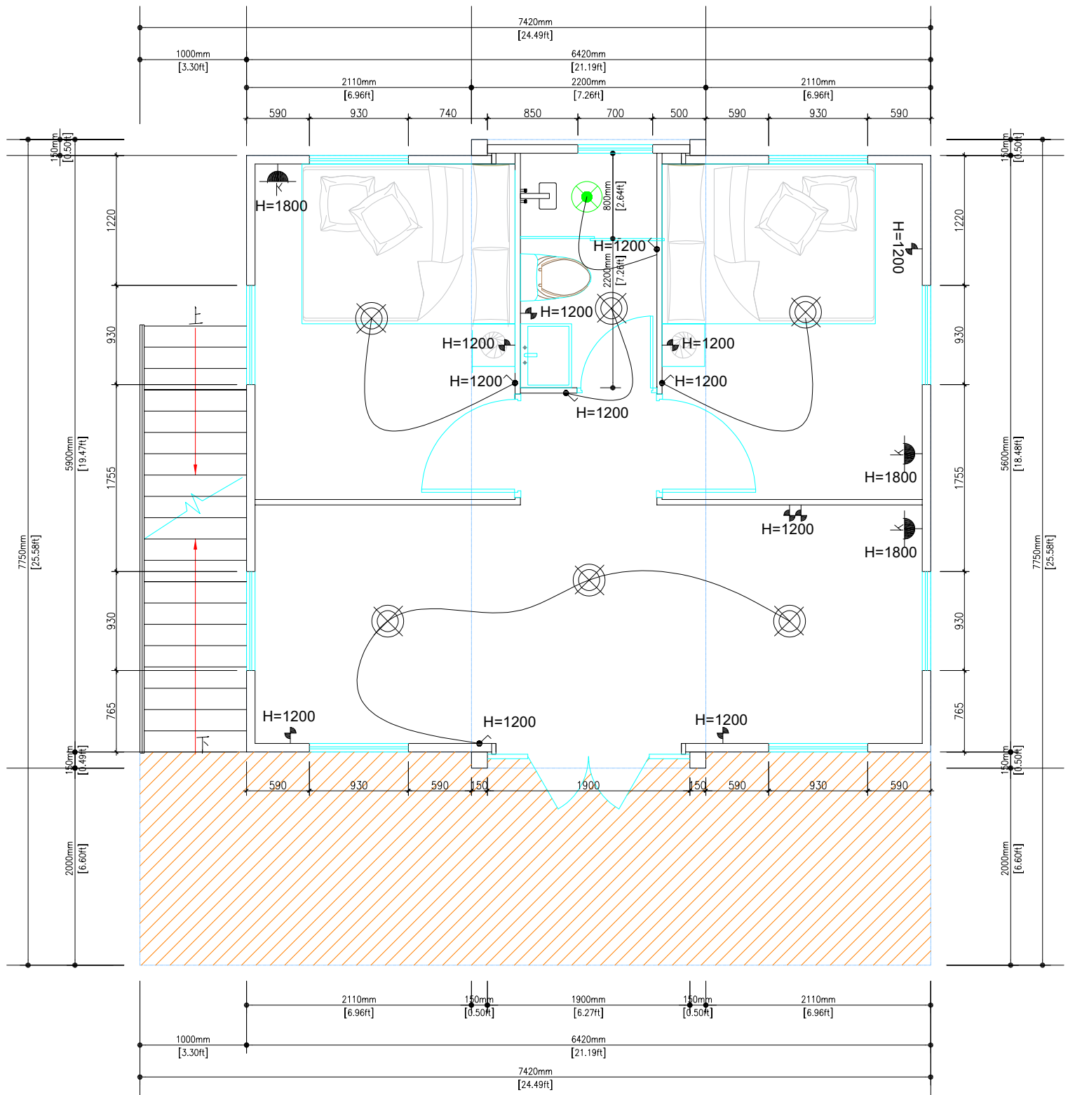
Second floor
