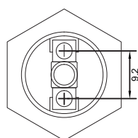
Screw terminal
