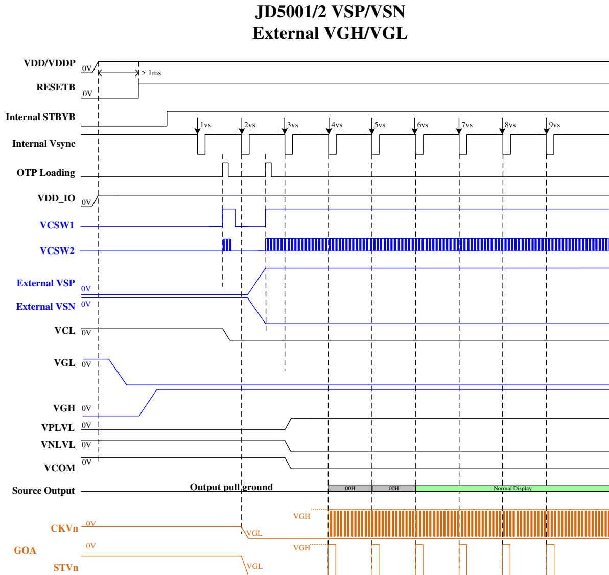
Figure 5.1: Power on sequence with PMODE[1:0]=00b
