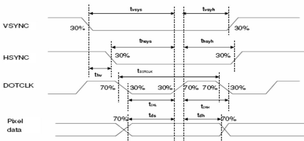
Figure 13. 1 Pixel Timing
