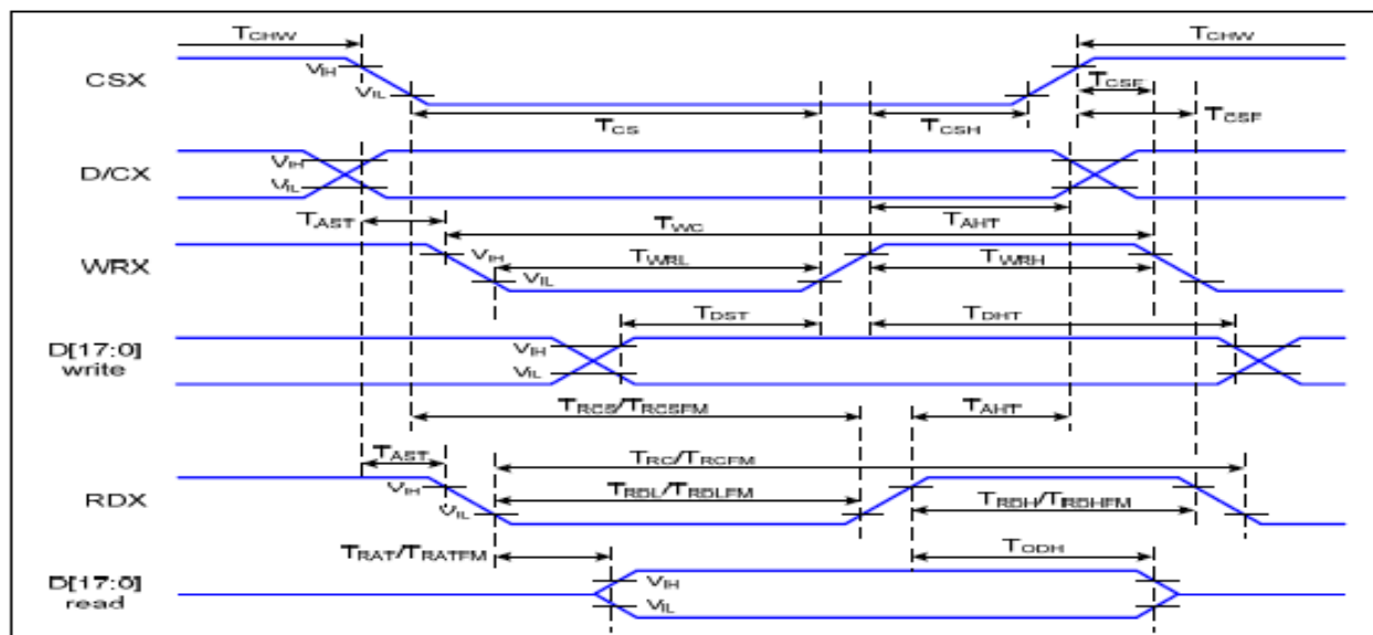
Figure 1 Parallel Interface Timing Characteristics (8080-Series MCU Interface)
