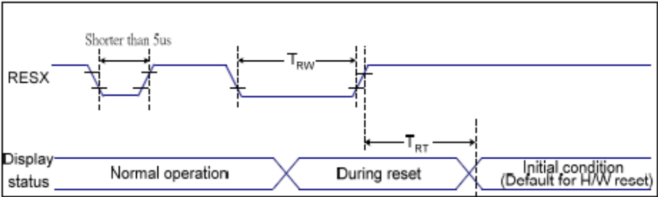
Figure 7 Reset Timing
