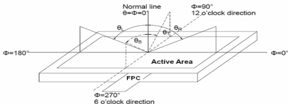
Fig. 1 Definition of viewing angle
