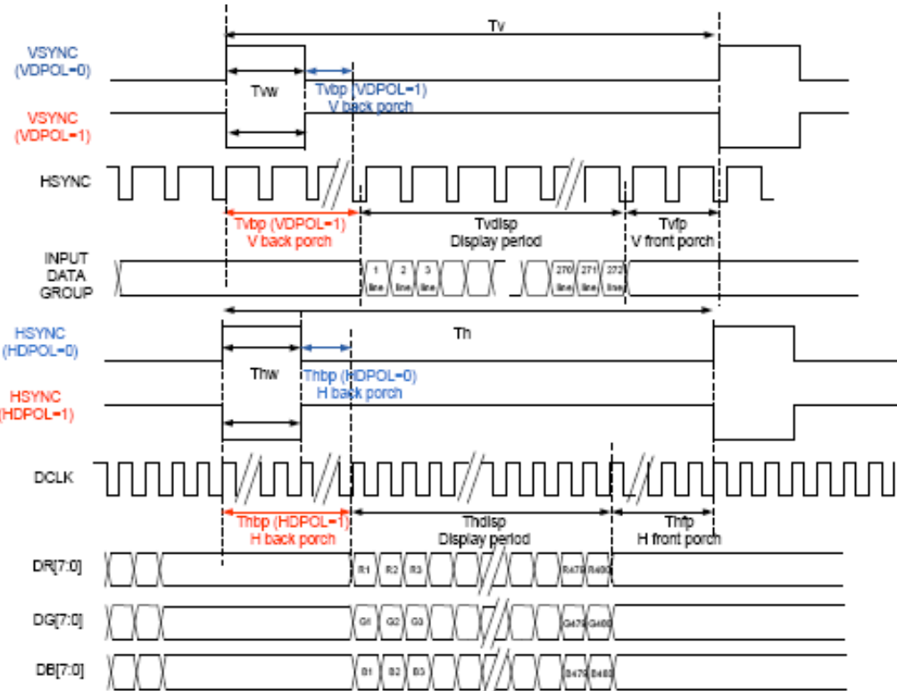
6.3 SYNC-DE Mode Timing Diagram
