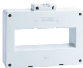
LMK3(BH)-0.66 200
