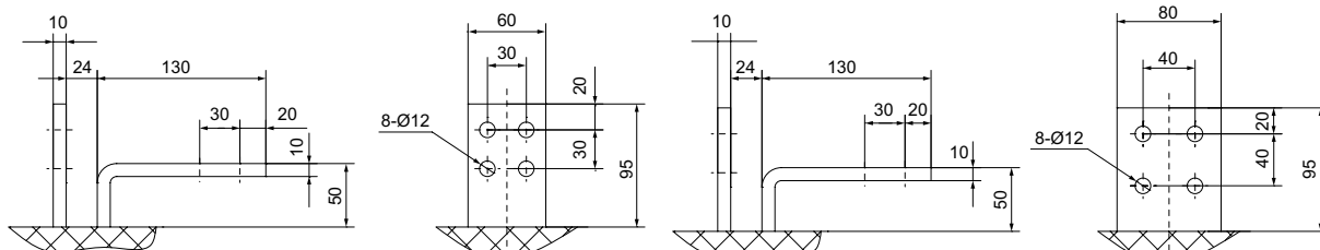
I1n=1200~2000A 时一次出线板尺寸 I1n=1200~2000A The size of the one-time output line board
