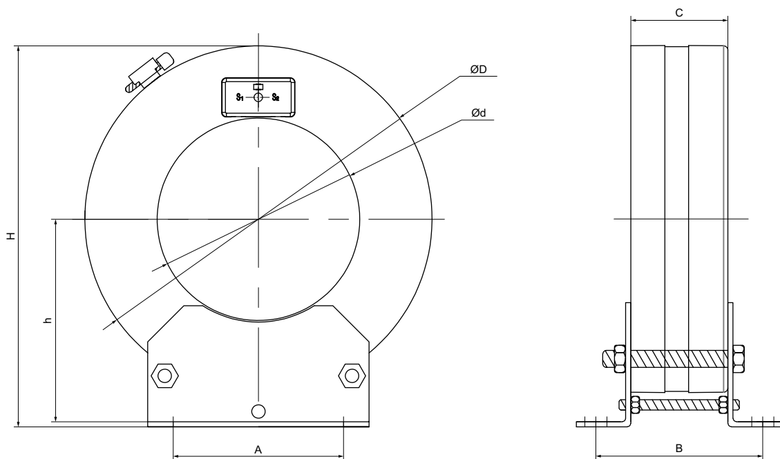
LXK-Ø80 系列零序电流互感器外形图及安装尺寸 LXK-Ø80 series Outline drawing and installation dimensions of zero-sequence current transformer
