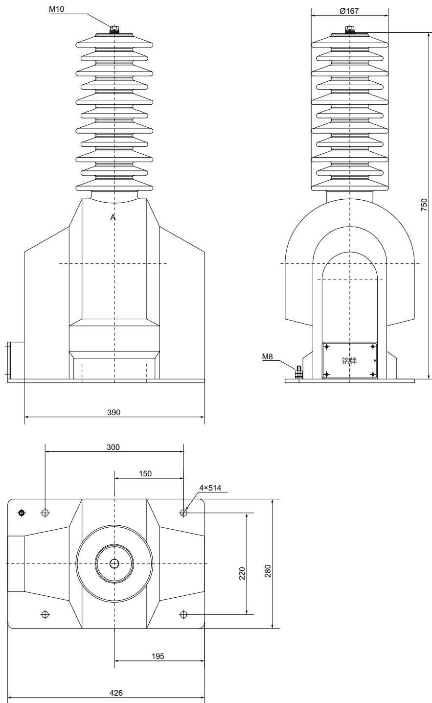
JDZXW9-35 型电压互感器外形图及安装尺寸 JDZXW9-35 Type voltage transformer outline drawing and installation dimensions
