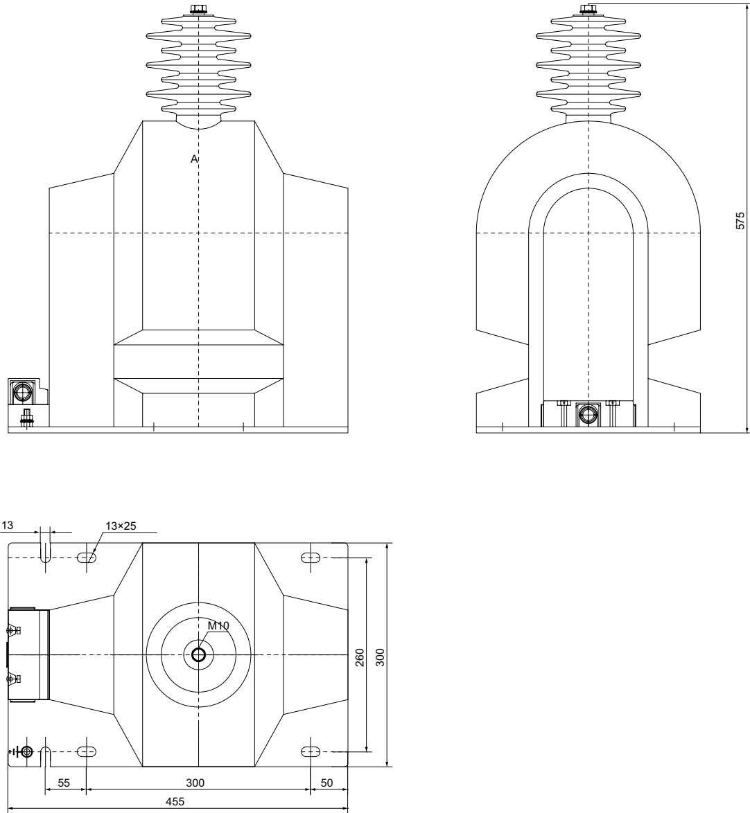
JDZXF14-35 型电压互感器外形图及安装尺寸 JDZXF14-35 type Voltage transformer outline drawing and installation dimensions
