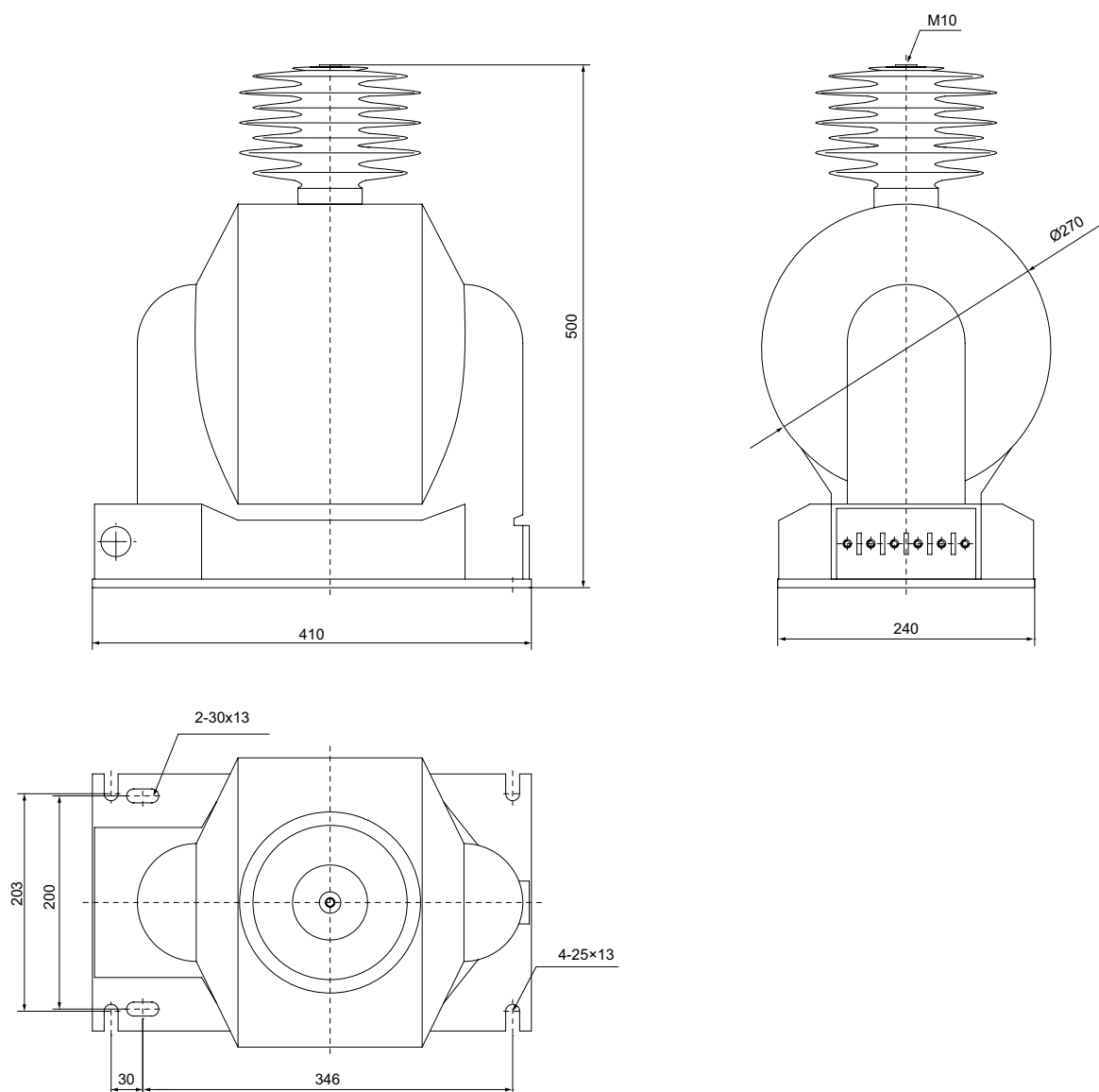
JDZX9-35 电压互感器外形图及安装尺寸 JDZX9-35 Voltage transformer outline drawing and installation dimensions
