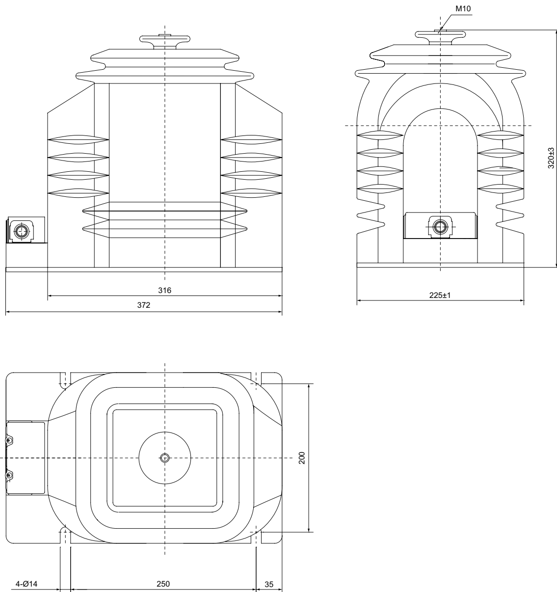
JDZX11-20 电压互感器外形图及安装尺寸 JDZX11-20 Voltage transformer outline drawing and installation dimensions
