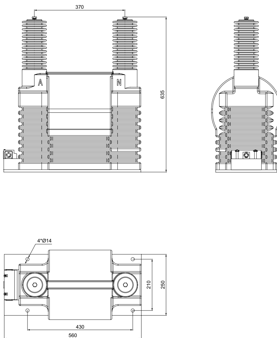
JDZ9-35 电压互感器外形图及安装尺寸 JDZ9-35 Voltage transformer outline drawing and installation dimensions
