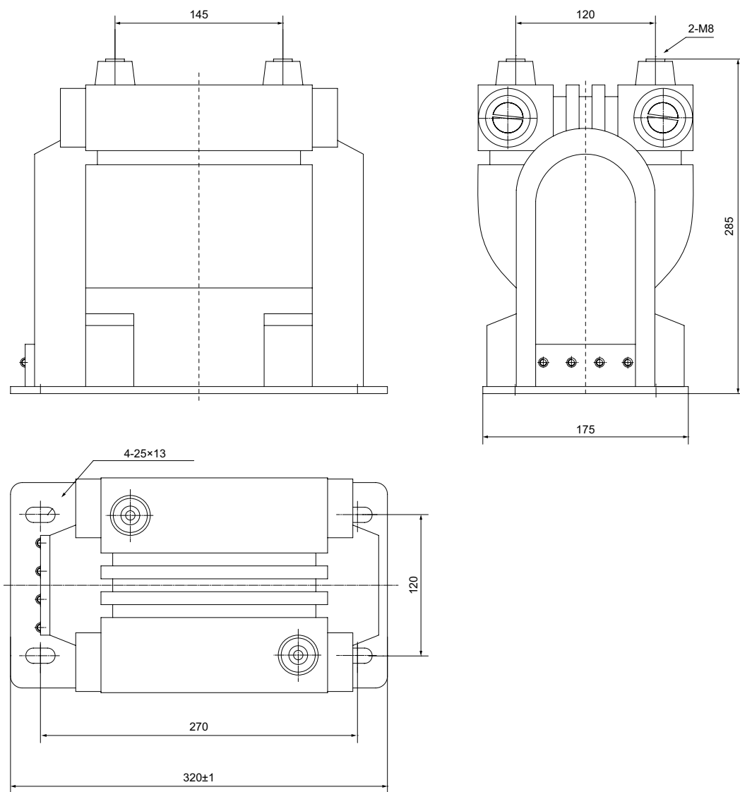
JDZ9-3、6、10R 电压互感器外形图及安装尺寸 JJZ9-3, 6, 10R Voltage transformer outline drawing and installation dimensions
