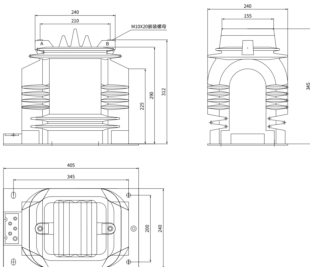
JDZ9-20 电压互感器外形图及安装尺寸 JDZ9-20 Voltage transformer outline drawing and installation dimensions
