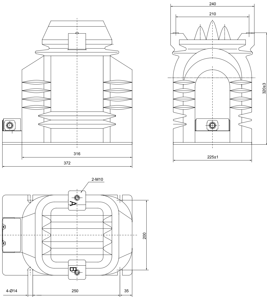
JDZ11-20 电压互感器外形图及安装尺寸 JDZ11-20 Voltage transformer outline drawing and installation dimensions
