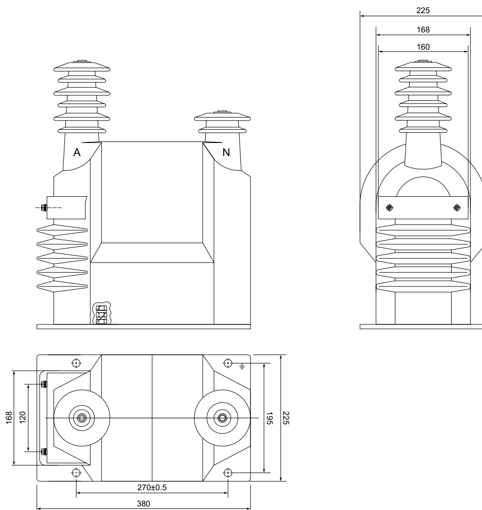
JDZ11-15 电压互感器外形及安装尺寸图 JDZ11-15 Voltage Transformer Outline and Installation Dimensions
