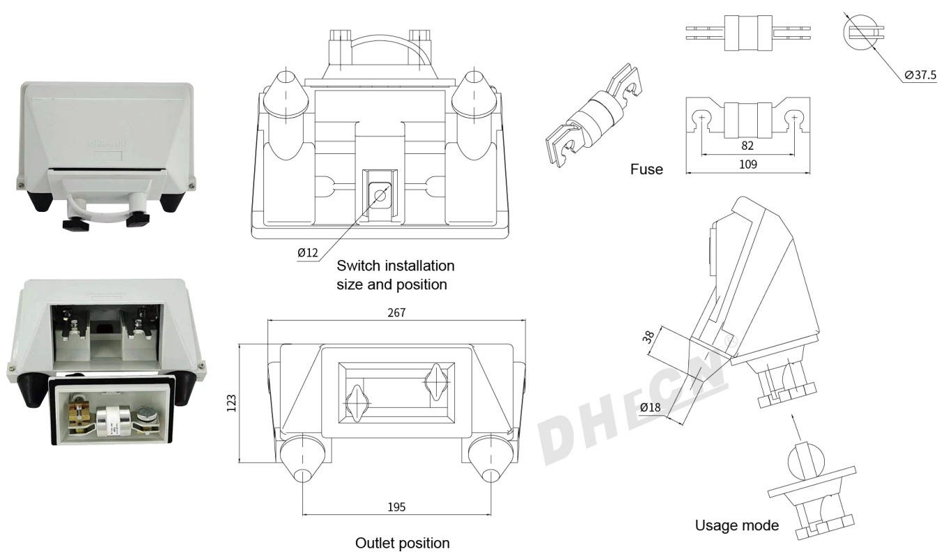
DHR-400 installation drawing
