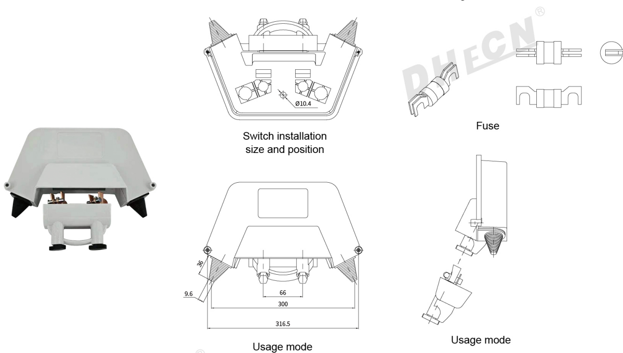
DHR-400B installation drawing
