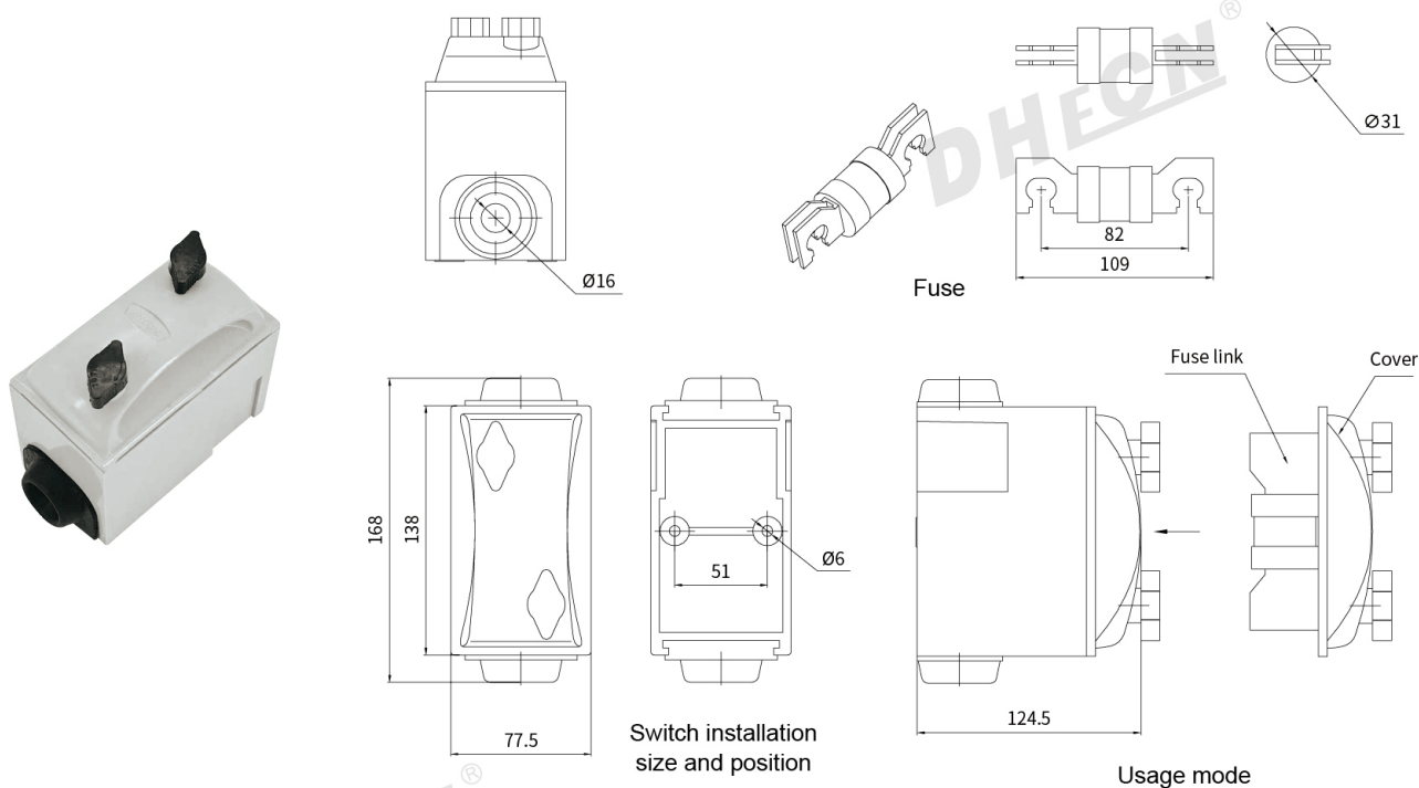
DHR-200 installation drawing
