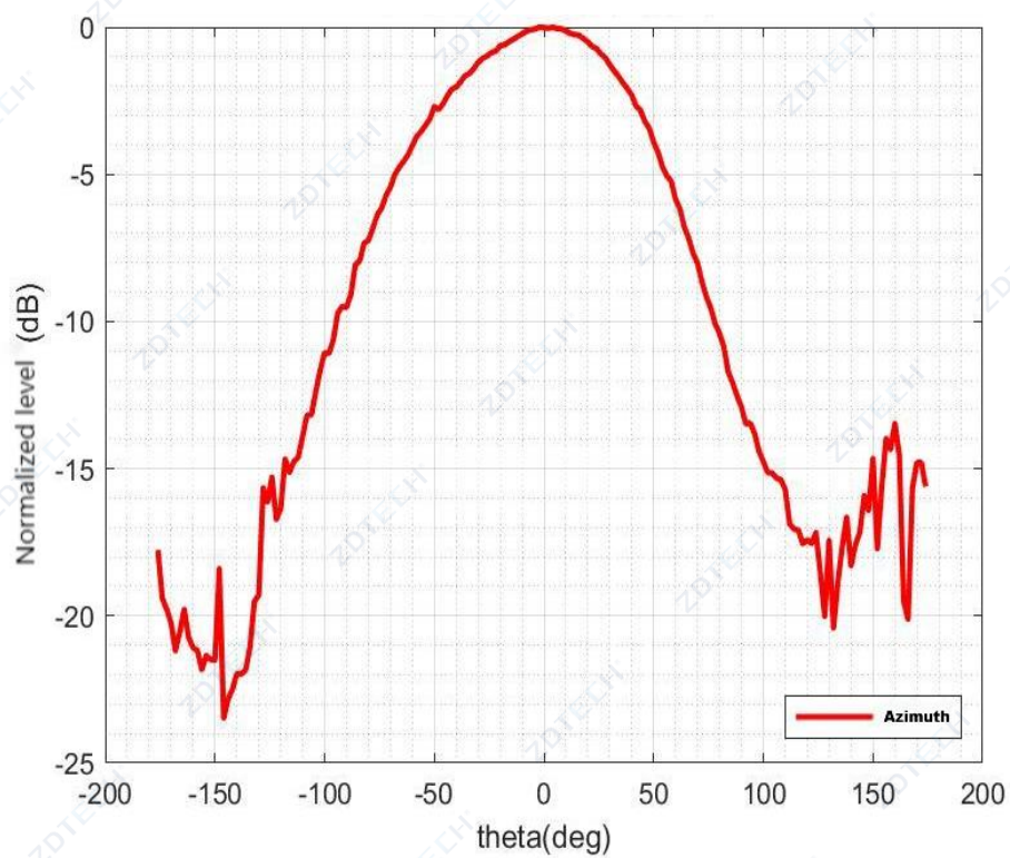
0.8GHz Directional Pattern
