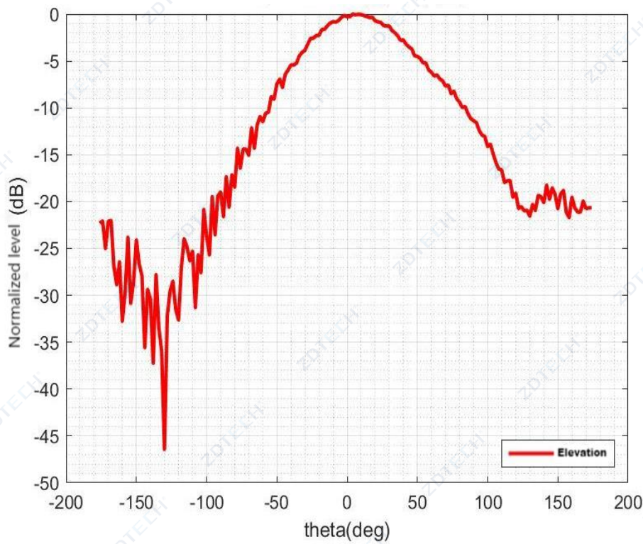
1.82GHz Directional Pattern
