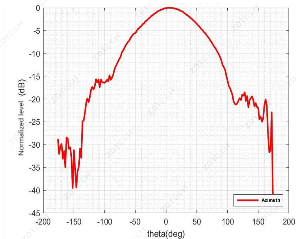
1.52GHz Directional Pattern
