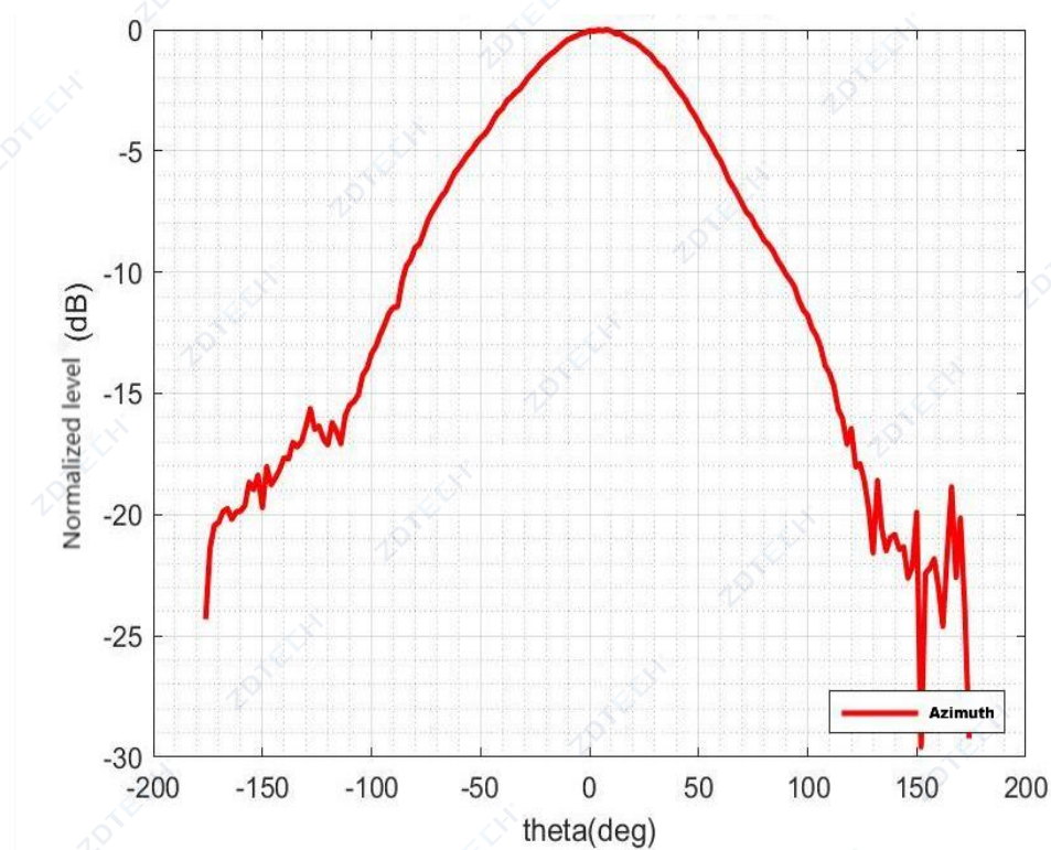
1.04GHz Directional Pattern
