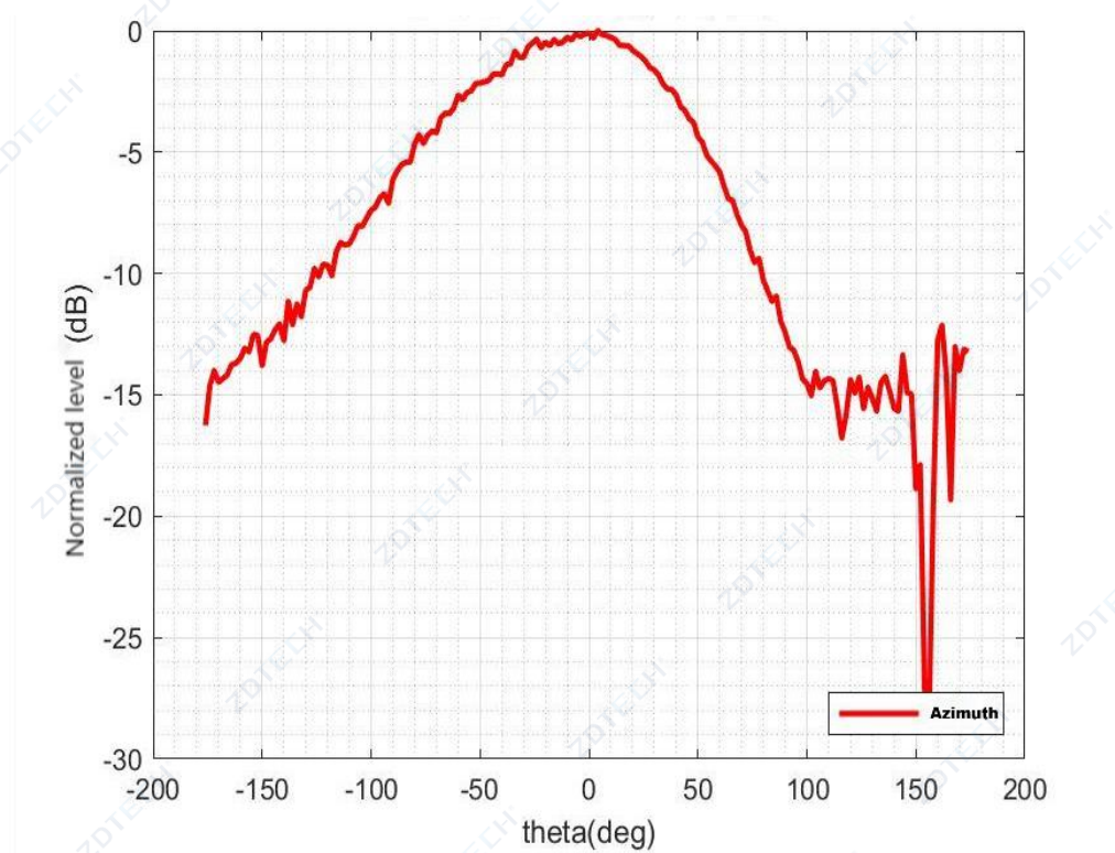
0.38GHz Directional Pattern
