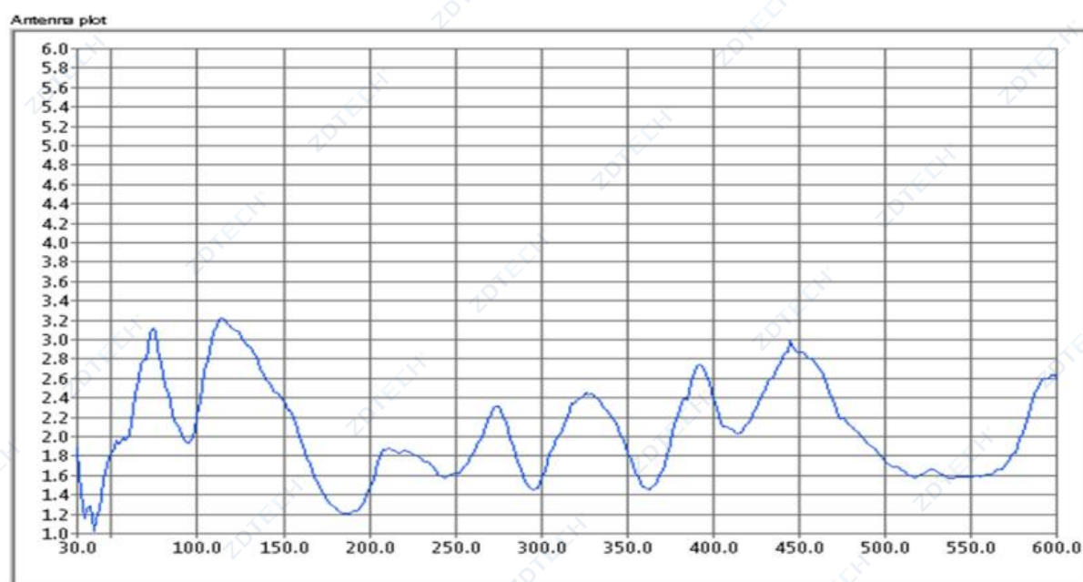
Typical VSWR Curve Antenna installed on the corner of a 3 x 3m ground plane
