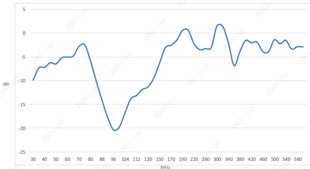
Antenna installed in the centre of a 3 x 3m ground plane
