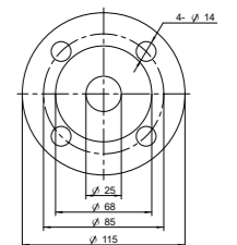
Fig 2. Flange Dimensions
