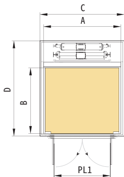
1 Minimum Shaft plan with 1 entrance [mm]
