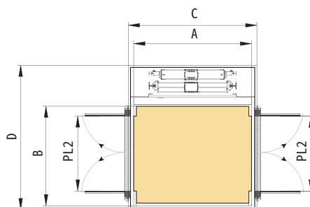
2 Minimum Shaft plan with through entrances [mm]
