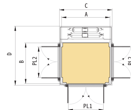
4 Minimum shaft dimensions with 3 entrance rear frame [mm]
