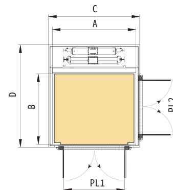
3 Minimum Shaft plan with 2 adjacent entrances [mm]
