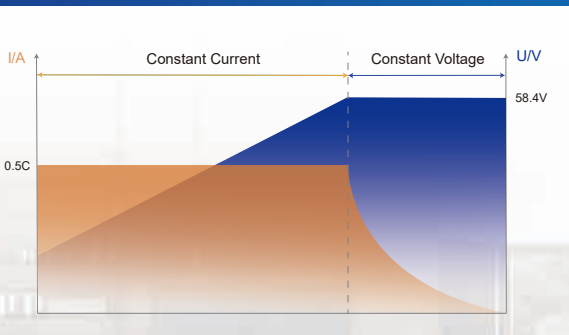
LiFePO4 Battery Charging Logic @0.5C
