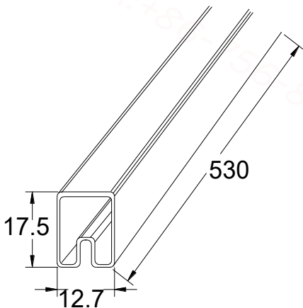
Tube: 530*17.5*12.7mm
