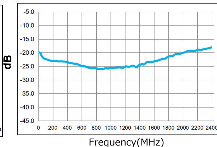
Output 2 Return Loss (Pin3)
