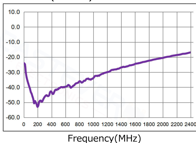
Isolation(Pin4-3)
