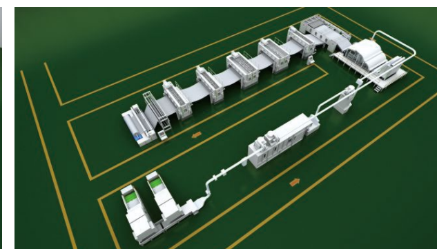
■ 针刺非织造布生产线 Needle-punching Nonwovens Production Line
