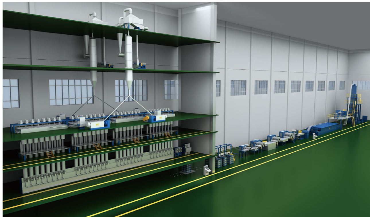
■ 涤纶短纤生产线 Complete Set of Polyester Staple Fiber Equipment
