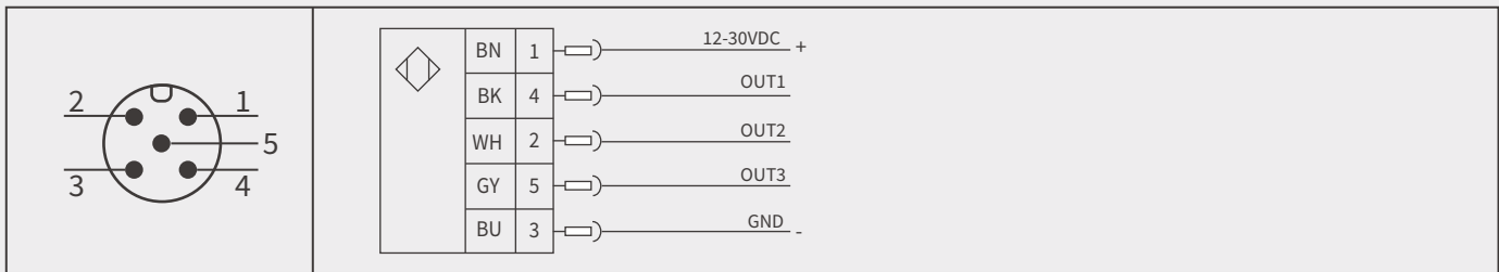
A3: Two switches + one analog (4-20mA)
