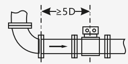
90°elbow
