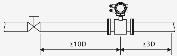
Valve is installed upstream of the sensor
