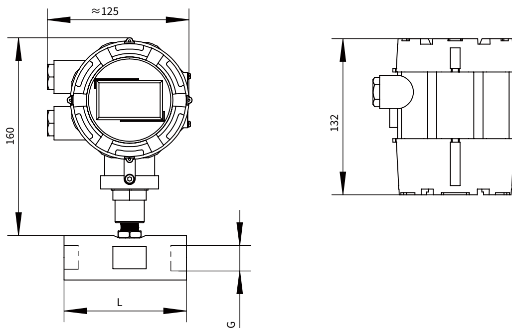
Dimension drawing(mm)
