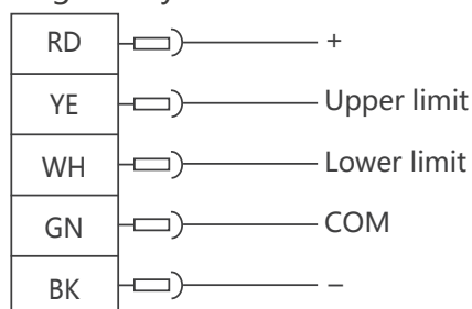
Single relay
