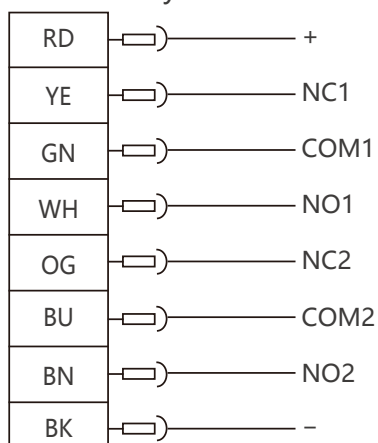
Double relay
