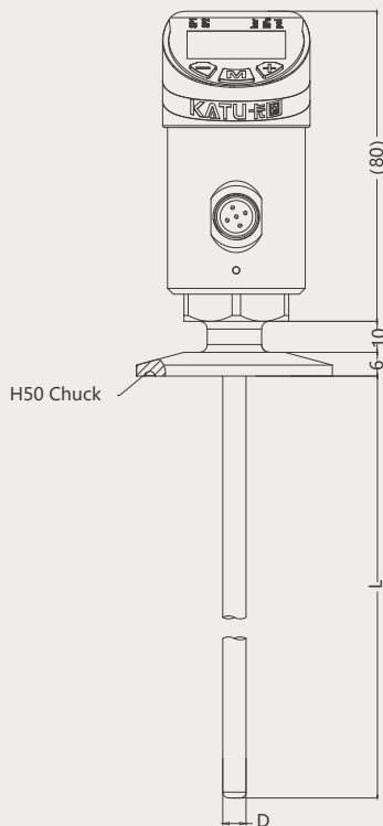
■ Standard chuck type connection
