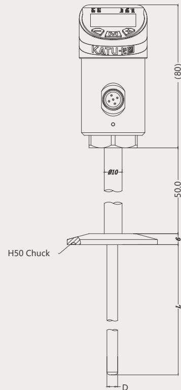
■ High and low temperature chuck type connection
