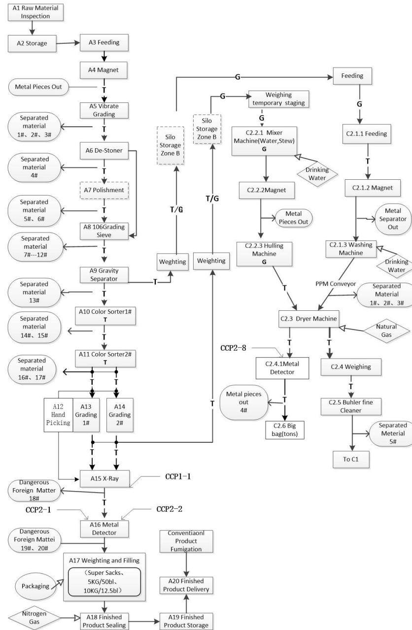
Flow Chart (A, C2 Zone for In shell Seeds Cleaning Hulling)
