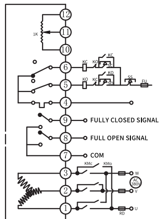
Type M: Three-phase AC 380V, with potentiometer and passive contact
