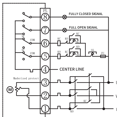
Type N: Three-phase AC 380V with source contact
