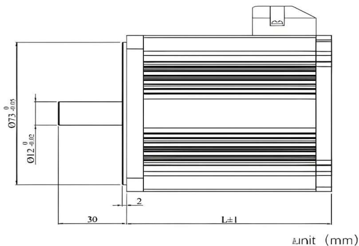
External Dimensions
