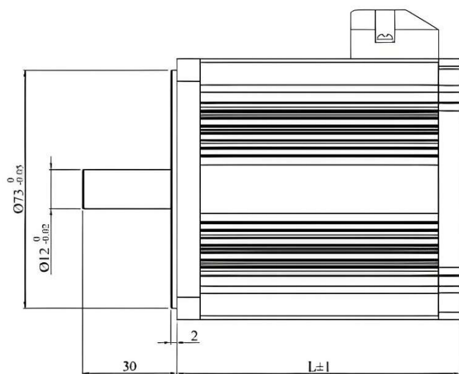
External Dimensions
