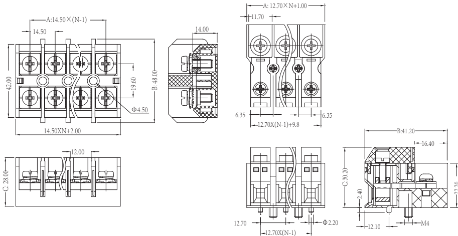
RTC60-XXP-B RTC60-XXP-C
