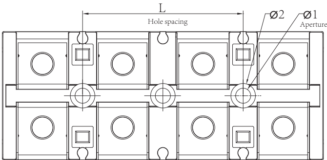
4-pole
