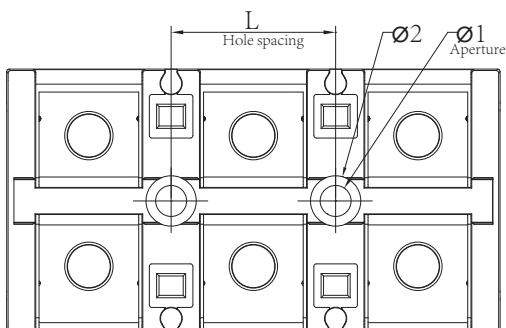
3-pole
