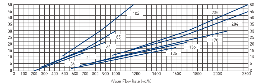
Water Flow Rate vs. Water Resistance Curve
