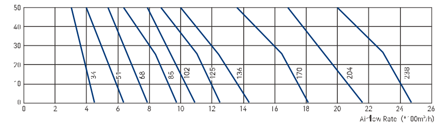
50Pa Unit Static Pressure and Airflow Characteristics
