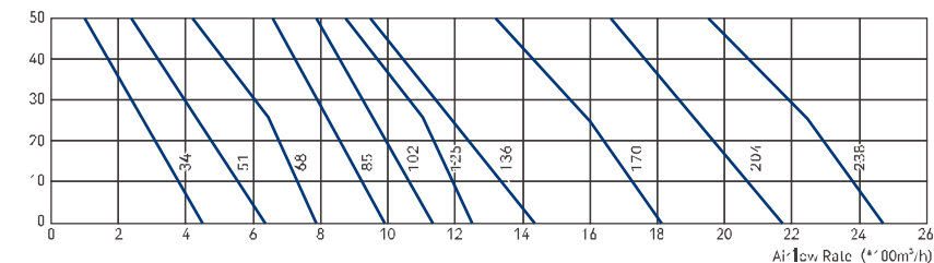
30Pa Unit Static Pressure and Airflow Characteristics
