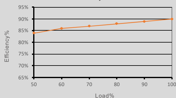
FSA-400W 24V
