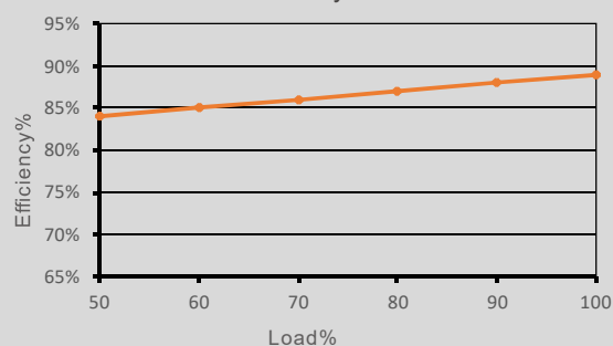
FSA-400W 12V
