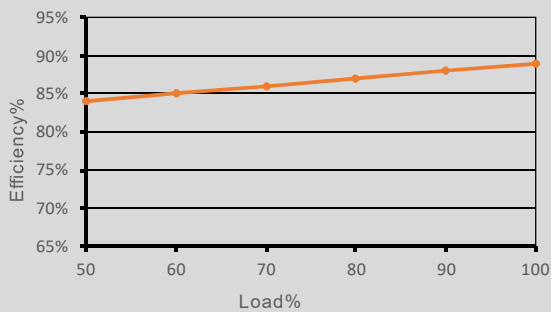
FSA-300W 12V
