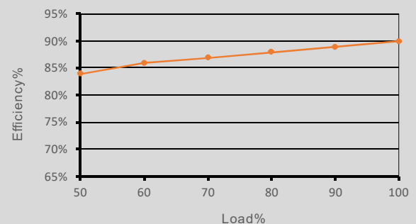
FSA-300W 24V
