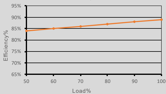
FSA- 150W 12V
