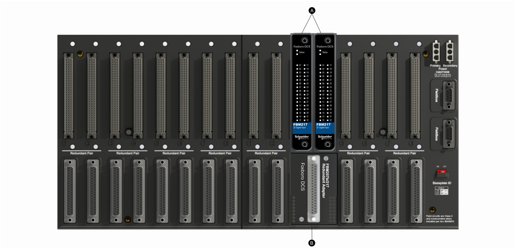
Figure 1 - Compact FBM217 Redundant Module Configuration
