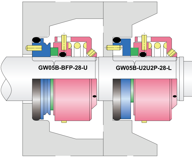
GW05B seal instead of AES T05B seal
