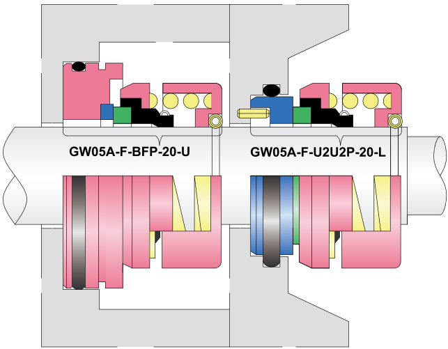
GW05A-F seal instead of original Flygt seal used for Flygt pump no: 2024/2066/2075/2101/3065/3080/Ready 24
