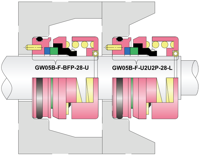
GW05B-F seal instead of original Flygt seal used for Flygt pump no: 3101
