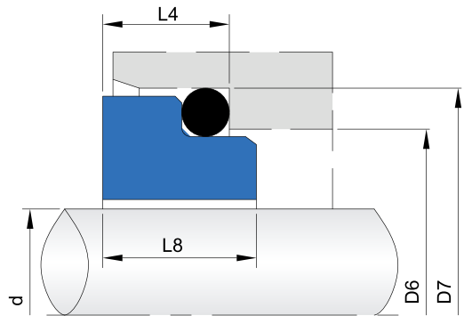
O-ring mounted seats, with standard dimensions. Material: V1, Q1, Q2, U2 A.B
