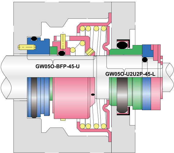
GW050 seal instead of AES T050 seal
