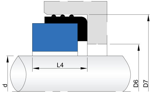
Cup mounted seats,according with DIN24960 standard. Material: V1, Q1, Q2, U2
