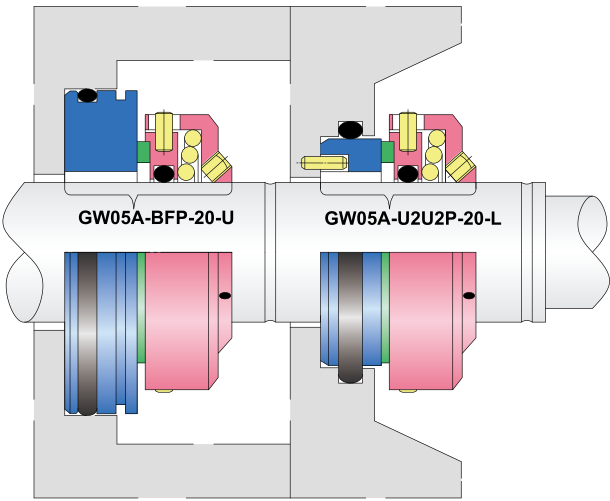
GW05A seal instead of AES T05A seal
