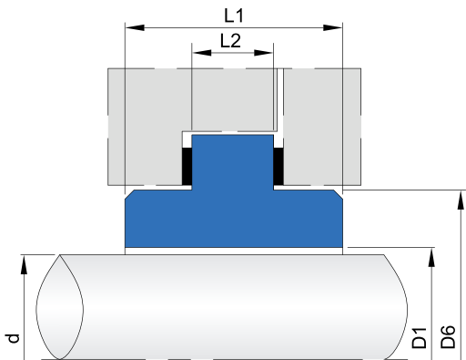
The seat with two PTFE gaskets should be clamped structure. Material: V1, Q1, Q2
