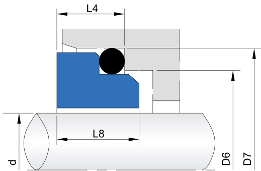
O-ring mounted seat,according with DIN 24960 standard. Material: V1, Q1, Q2, U2
