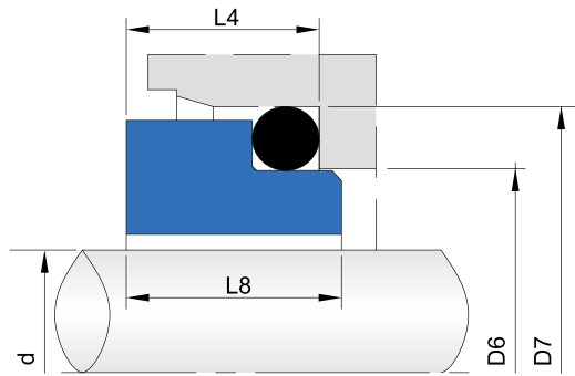
O-ring mounted seats. according with DIN24960 standard. Material: V1, Q1, Q2, U2
