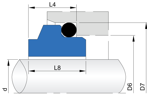
O-ring mounted seats. with a short axial dimension. Material: V1, Q1, Q2, U2 A.B
