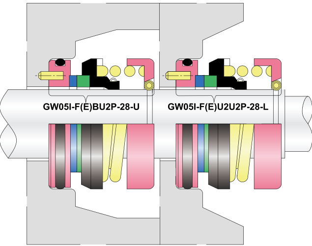
GW05I-F(E) seal and GW05I-F(L) seal instead of original Flygt seal used for Flygt pump no: 2082/2090/2125/2140/Ready 90
