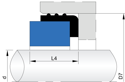
Cup mounted seats,according with DIN24960 standard. Material: V1, Q1, Q2, U2
