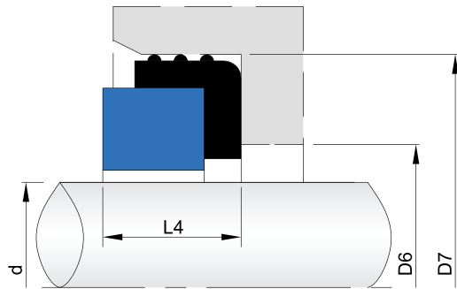
Cup mounted seats,according with DIN24960 standard. Material: V1, Q1, Q2, U2
