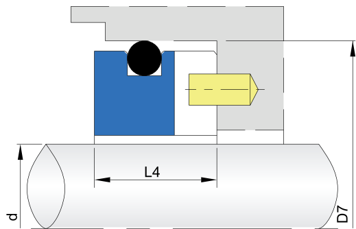
O-ring mounted seats.with anti-rotation slot, can apply to common Euripean standard seals housing dimensions. Material: V1, Q1, Q2, U2
