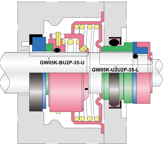
GW05K seal instead of AES T05K seal
