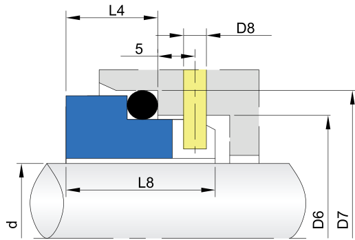
O-ring mounted seats. with anti-rotation pin, according with DIN24960 standard. Material: V1, Q1, Q2, U2
