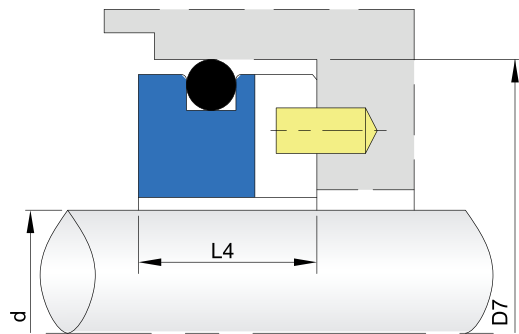
O-ring mounted seats.with anti-rotation slot, can apply to American standard seals housing dimensions. Material: V1, Q1, Q2, U2
