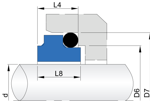
O-ring mounted seats. with a standard dimensions. Material: V1, Q1, Q2, U2 A.B
