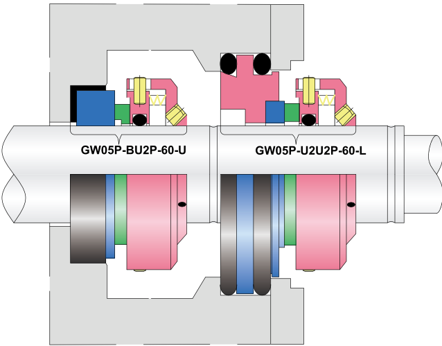
GW05P seal instead of AES T05P seal
