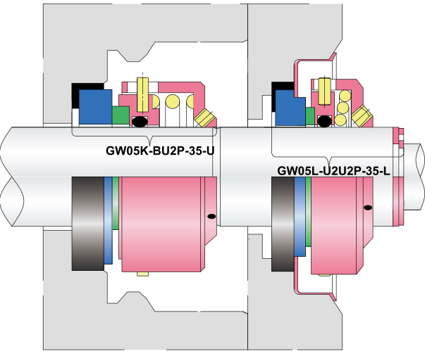
GW05KL seal instead of AES T05KL seal
