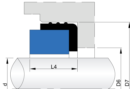
Cup mounted seats,according with DIN24960 standard. Material: V1, Q1, Q2, U2
