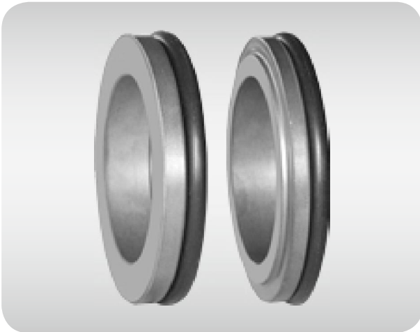
O-ring mounted seat, according with DIN 24960 standard. Material: V1, Q1, Q2, U2 A.B
