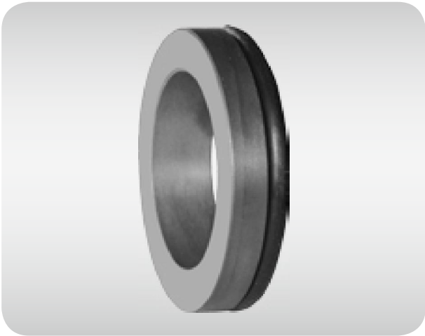
O-ring mounted seat,according with DIN 24960 standard. Material: V1, Q1, Q2, U2
