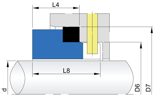
PTFE rectangular ring mounted seats. with anti-rotation pin, according with DIN24960 standard. Material: V1, Q1, Q2, U2
