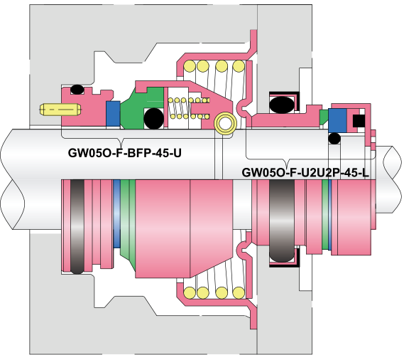
GW050-F seal instead of original Flygt seal used for Flygt pump no:2201-011 LT/3140/3152/4650/4660
