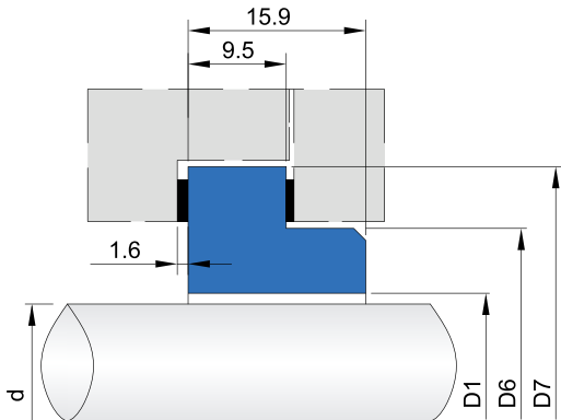
The seat with two PTFE gaskets design with L-shape profile. It can be fitted in Multiple-Spring balanced seals. Material: V1, Q1, Q2
