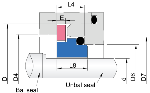
O-ring mounted seats. according with DIN 24960 standard. with seat blocked ring and suitable for vacuum application. Material: V1, Q1, Q2, U2
