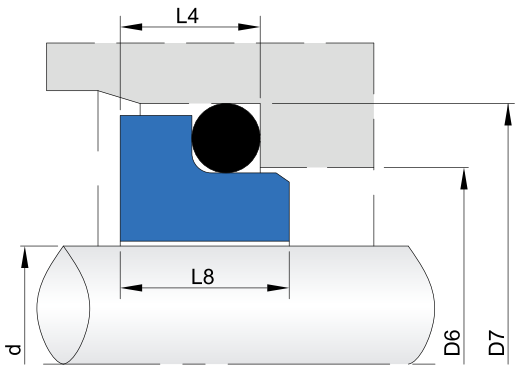
O-ring mounted seats.with short design according with DIN24960 standard. Material: V1, Q1, Q2, U2
