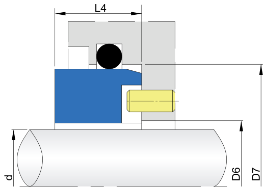
O-ring mounted seats. according with DIN24960 standard. Material: V1, Q1, Q2, U2
