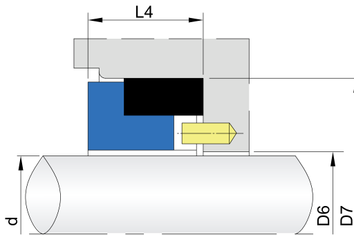
PTFE rectangular ring mounted seats. with anti-rotation pin, according with DIN24960 standard. Material: V1, Q1, Q2, U2
