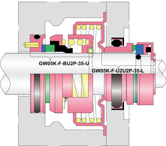
GW05K-F seal instead of original Flygt seal used for Flygt pump no: 2151-010/3126-090/3126-180
