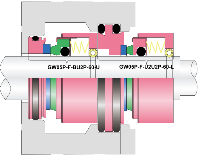
GW05P-F seal instead of original Flygt seal used for Flygt pump no:2250/2290/3200
