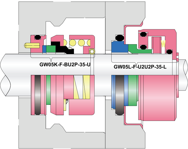
GW05KL-F seal instead of original Flygt seal used for Flygt pump no:2084/ 2135/2151-011/2151-050
