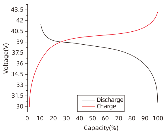
38.4V 100Ah Charge-Discharge Curve 0.5C, 25°C
